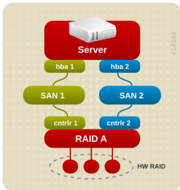
图 1.1. Active/Passive Multipath Configuration with One RAID Device
