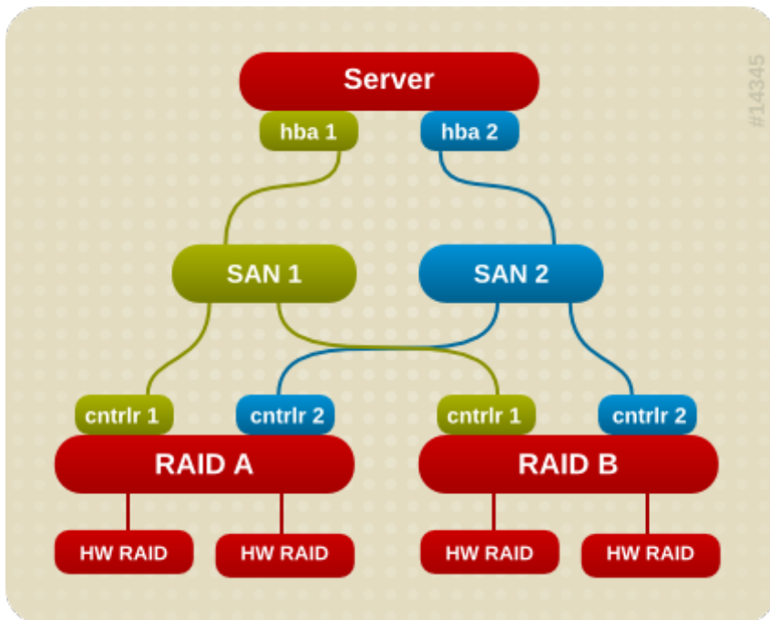
图 1.2. Active/Passive Multipath Configuration with Two RAID Devices
